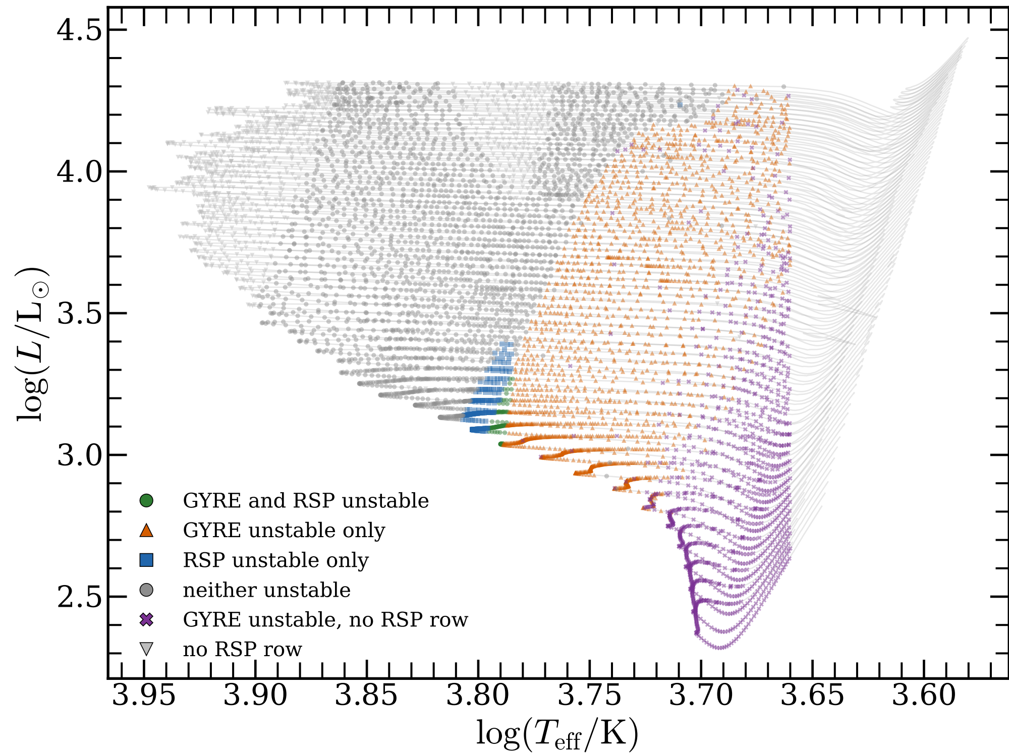
First-overtone instability classification ( F_1 > 0 )
