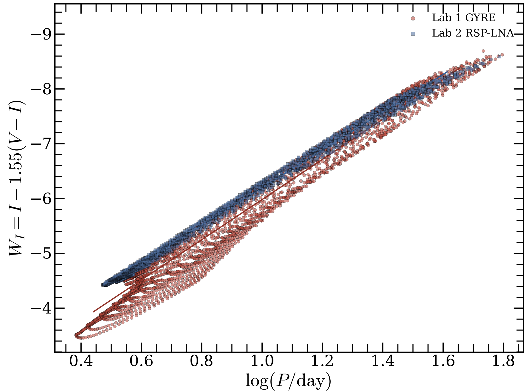
F_0 unstable period-Wesenheit relation
