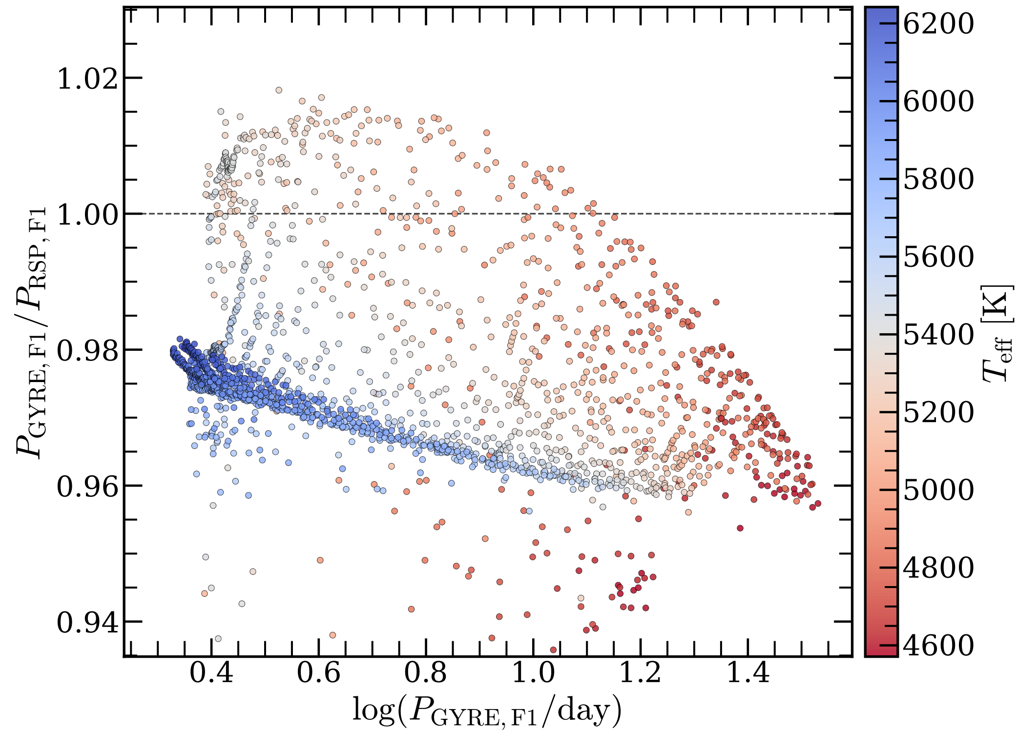
F_1 period ratio, GYRE-unstable matched models
