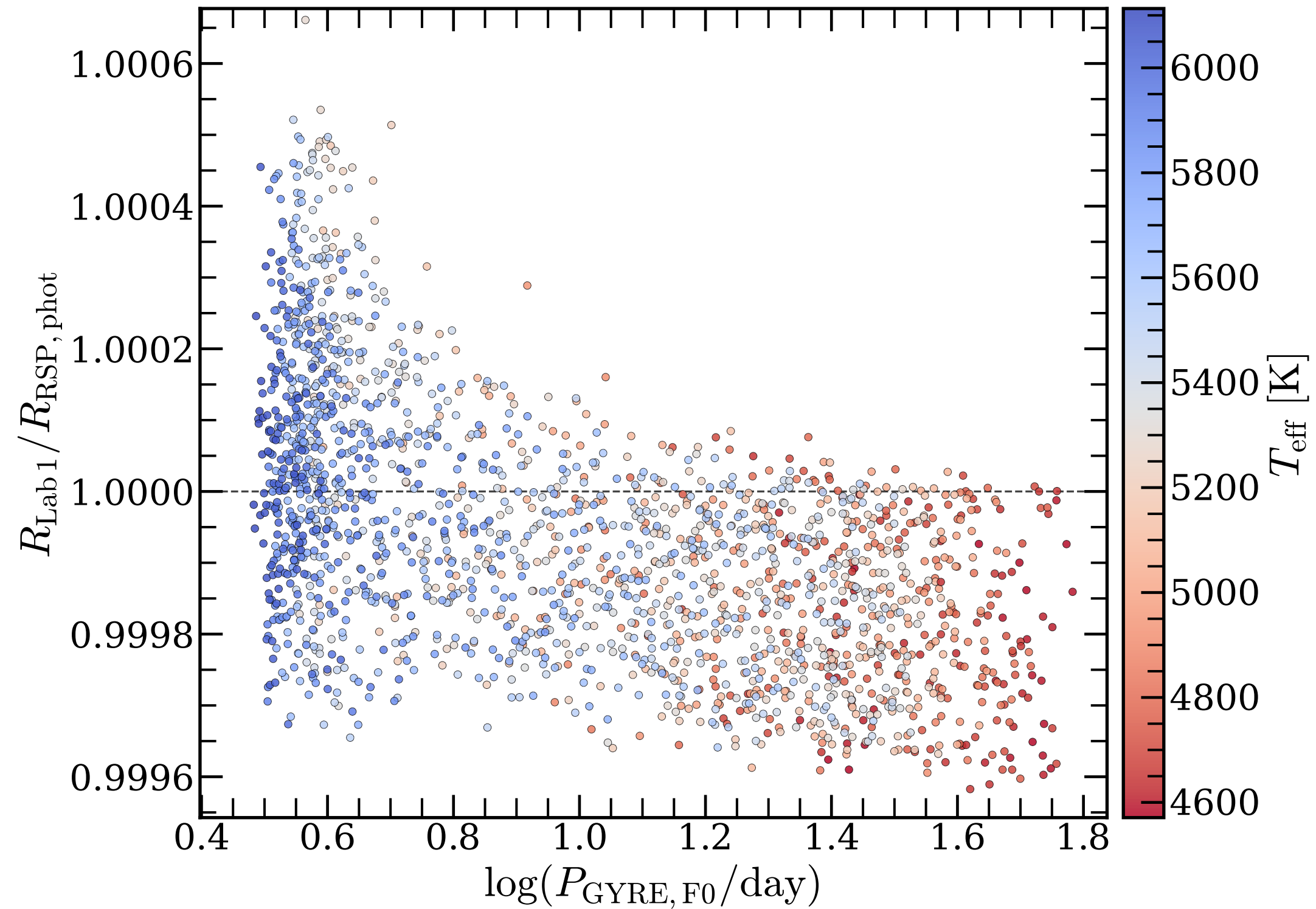
F_0 radius ratio, GYRE-unstable matched models
