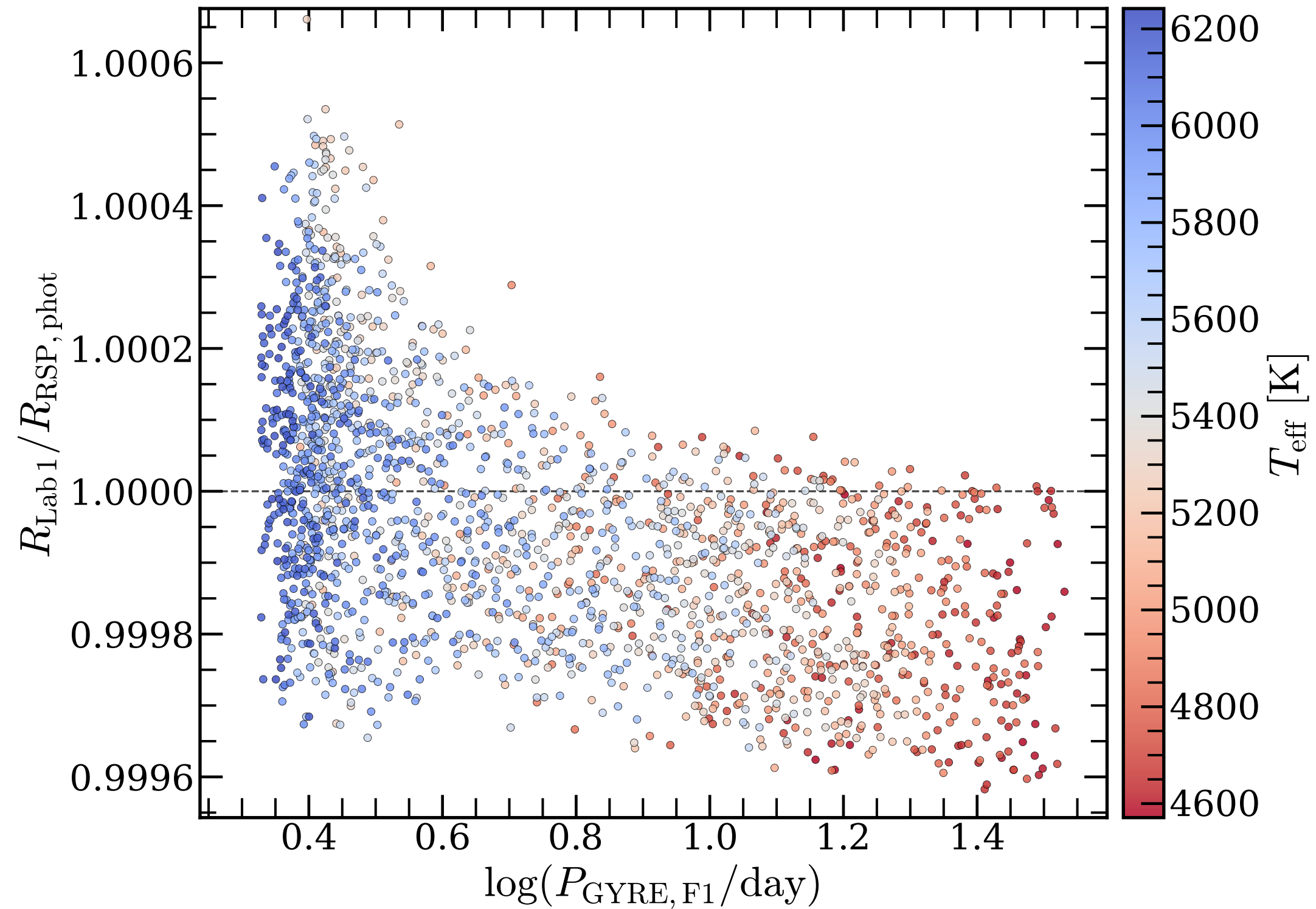
F_1 radius ratio, GYRE-unstable matched models
