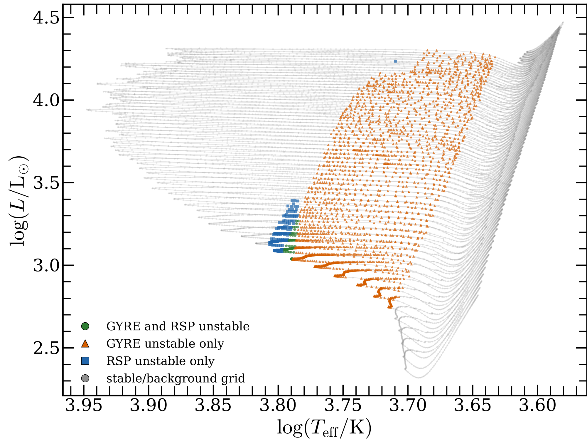
First-overtone classification (GYRE F_1 > 0 , F_2 subdominant)
