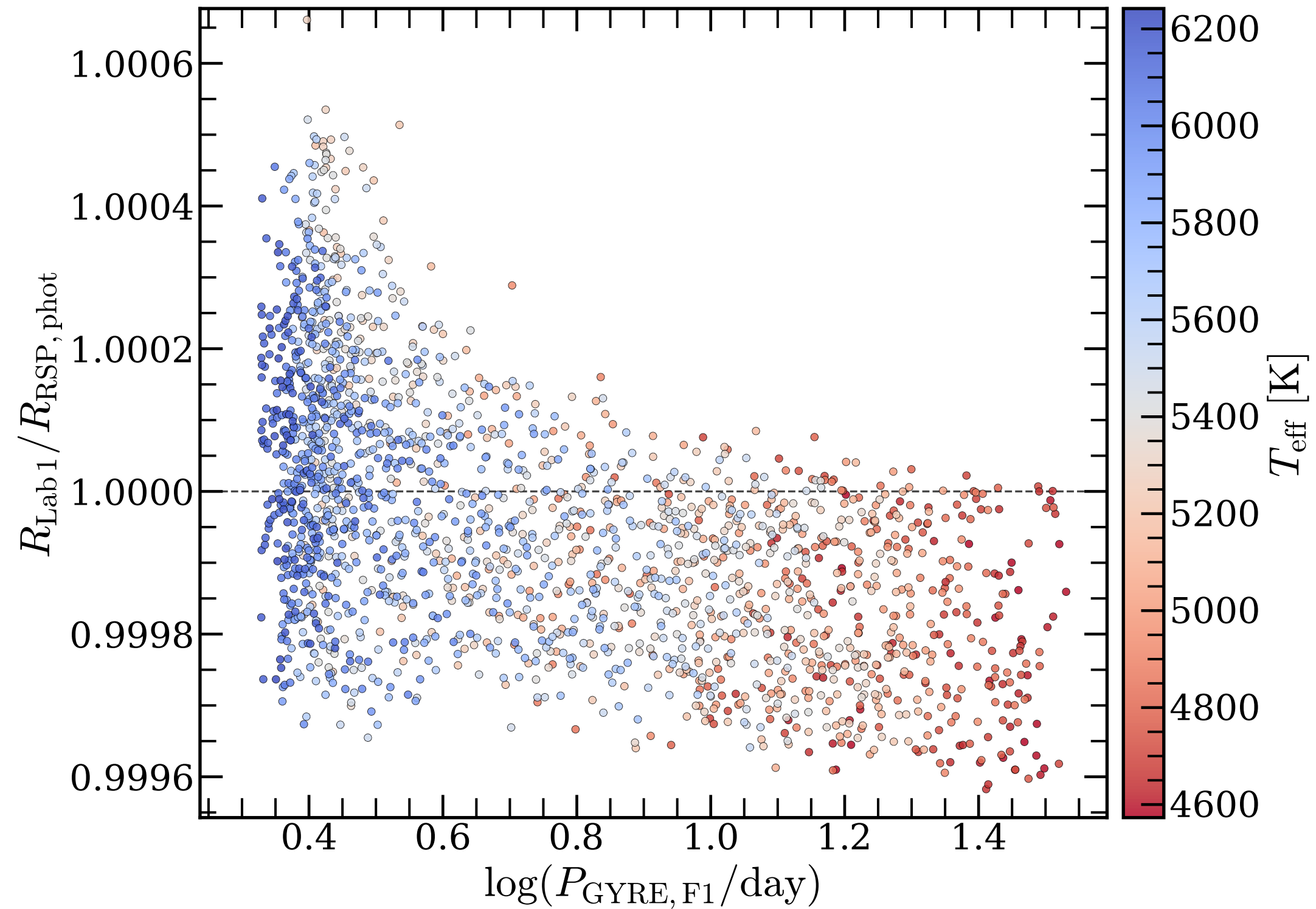
F_1 radius ratio, GYRE F_2 -subdominant matched models
