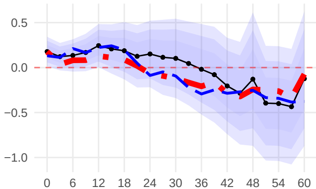
Intercept
