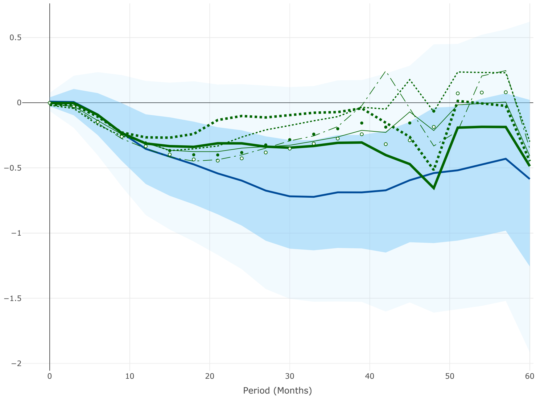
Average IRF for employment
