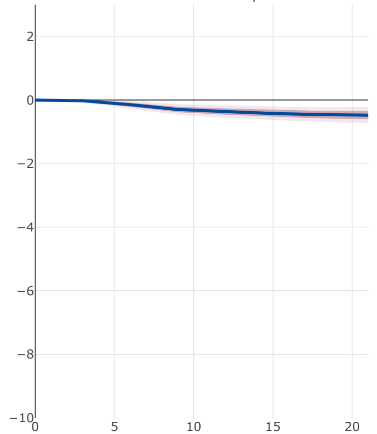
Cholesky
