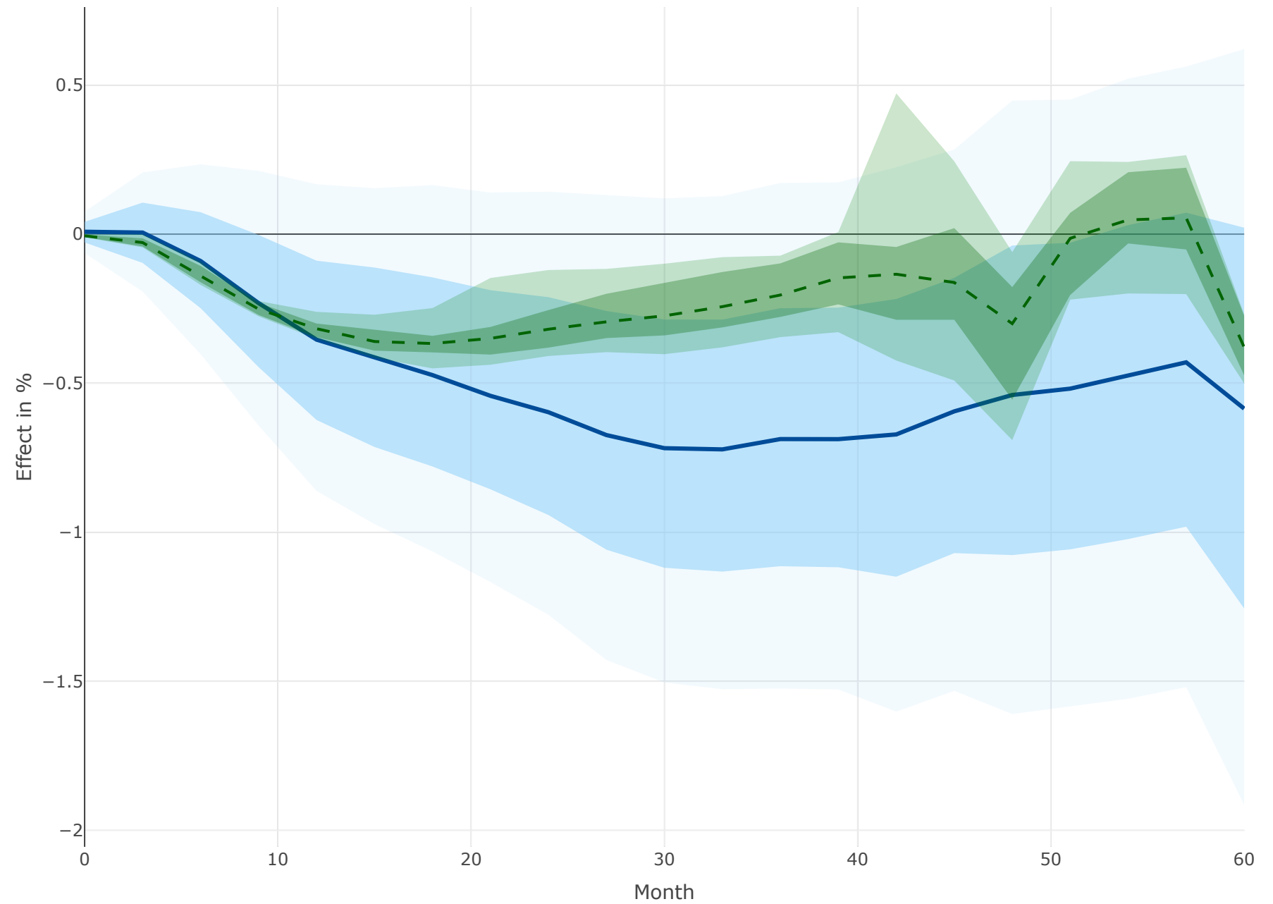
emp response to 100 bp rate shock, average and p-bias corrected range
