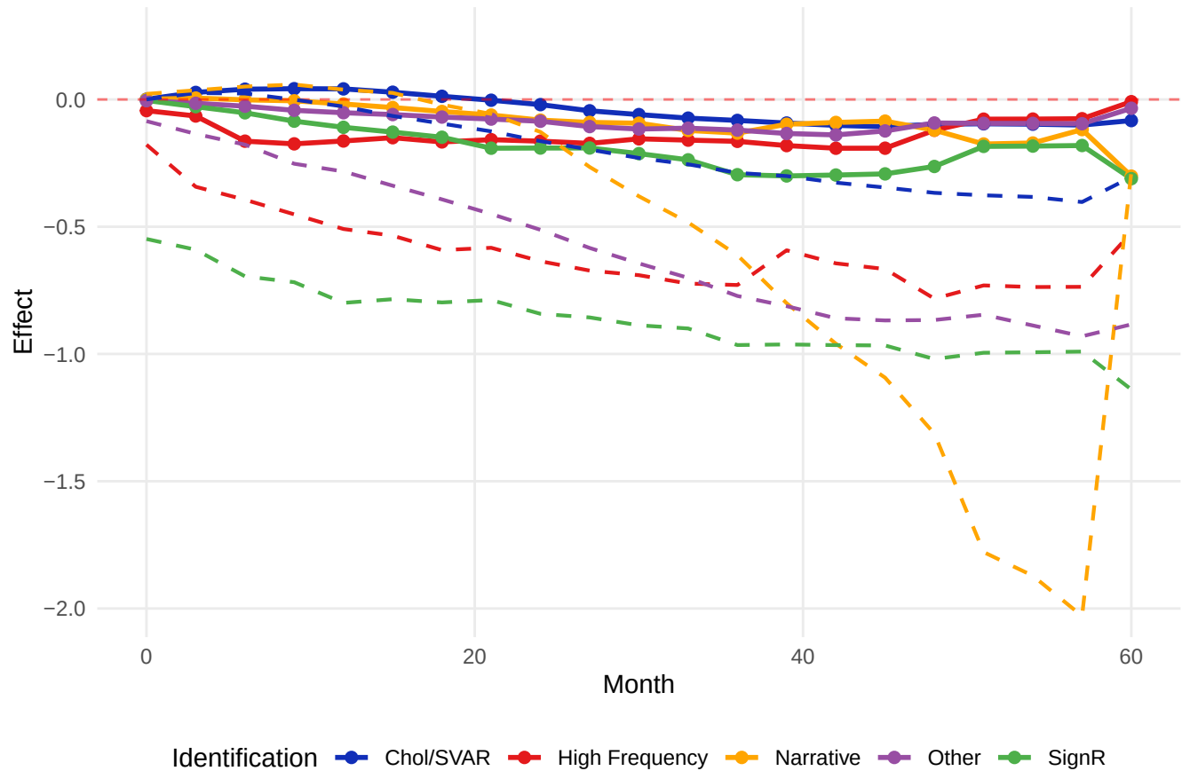
P-bias corrected effects assuming 14 % top journal, 54 % CB affiliation
