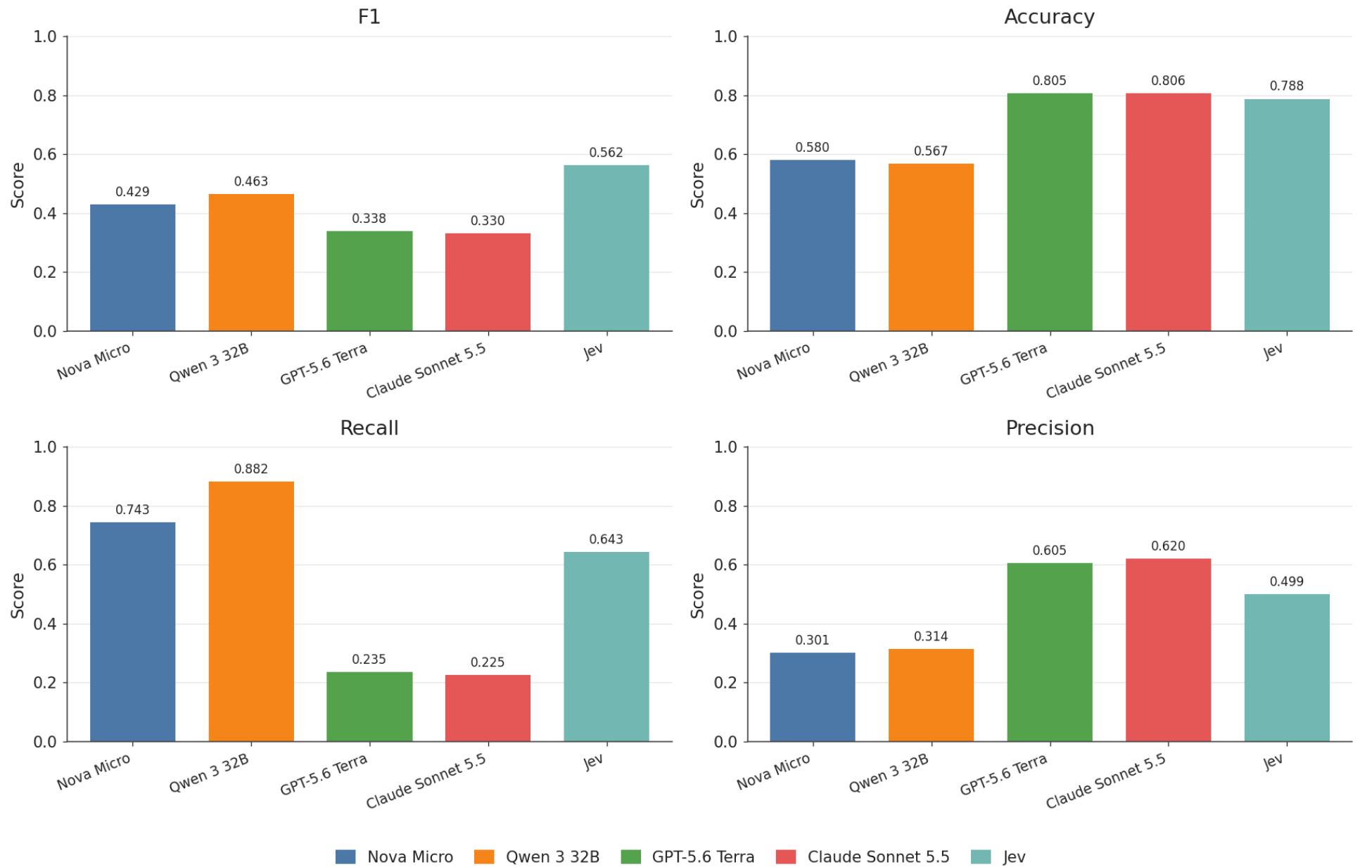
Figure 14: Few-shot baselines across all posts
