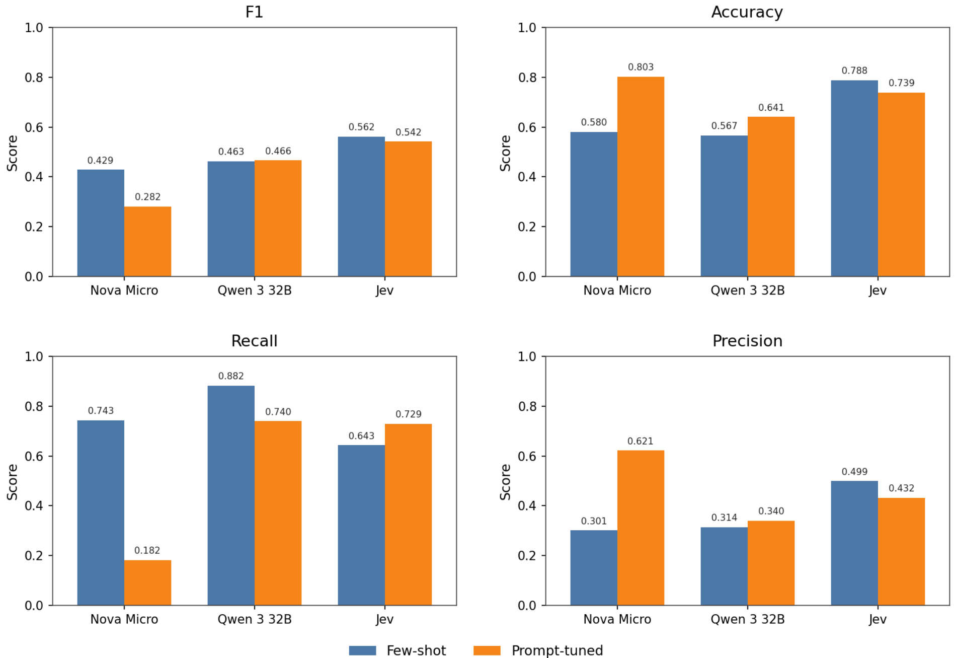
Figure 15: Prompt tuning vs few-shot — across all posts
