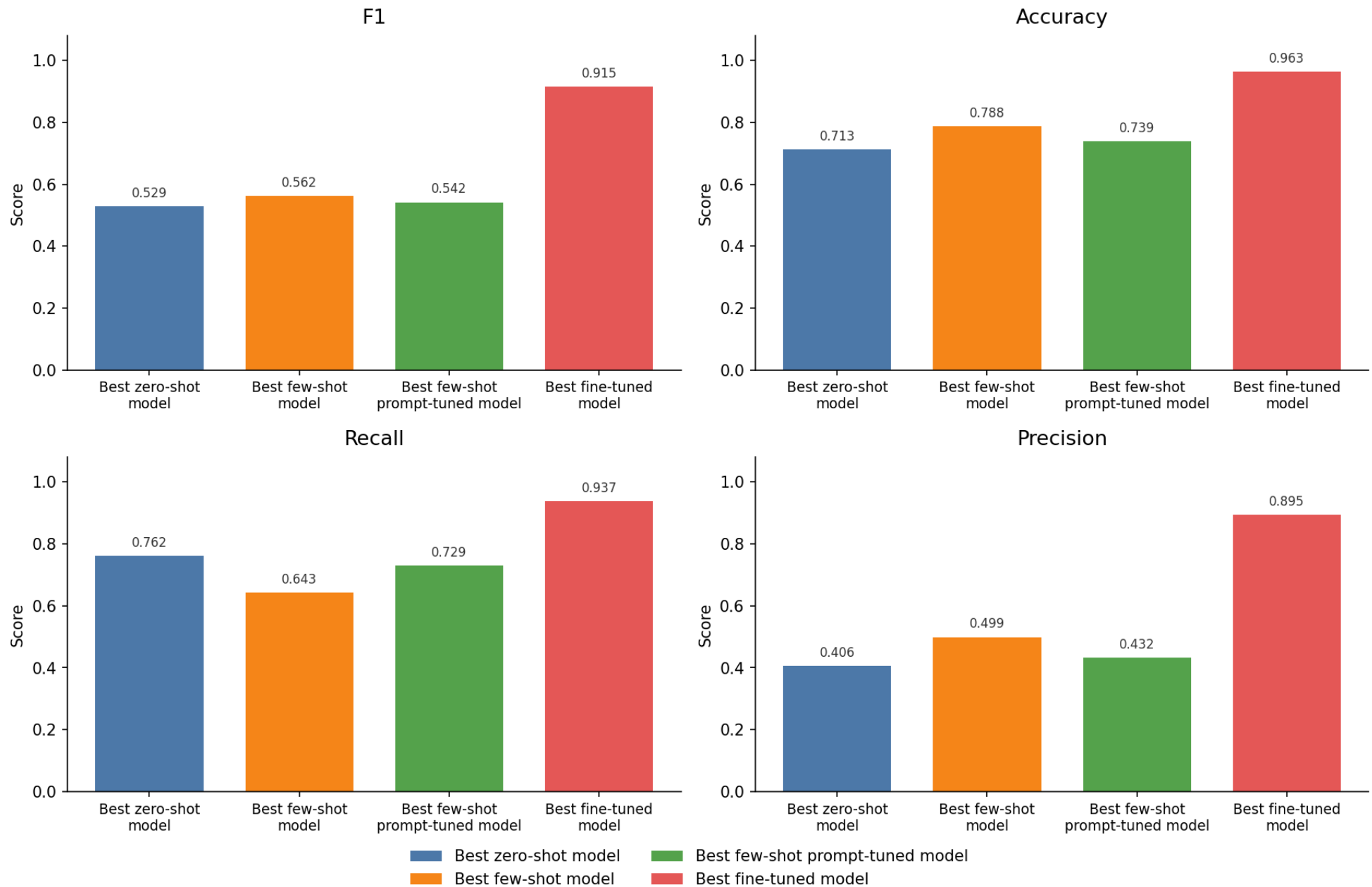
Figure 16: Fine-tuning outperforms prompt-based approaches
