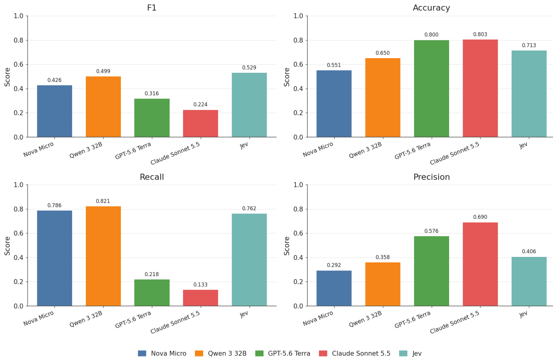
Figure 12: Zero-shot baselines across all posts
