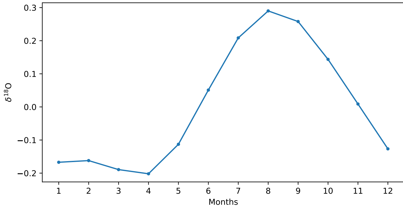
Climate Average for \delta^{18}\text{O}
