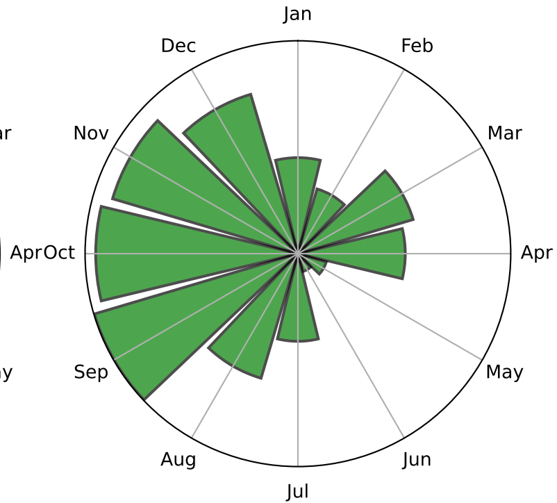
observed \delta^{13}\text{C}
