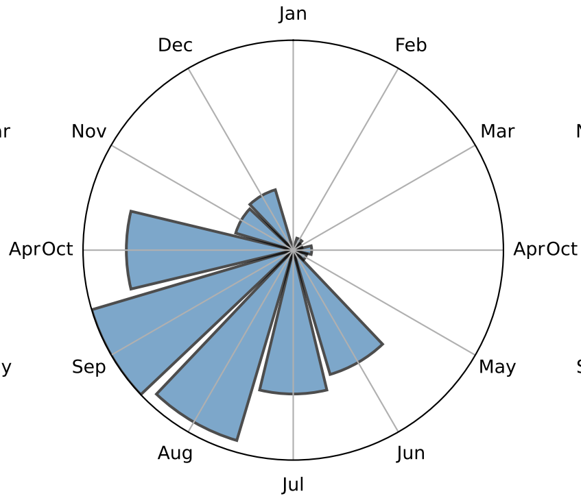
observed \delta^{18}\text{O}
