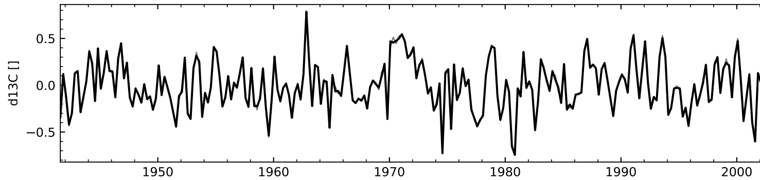
a) d13C without tectonic signal
