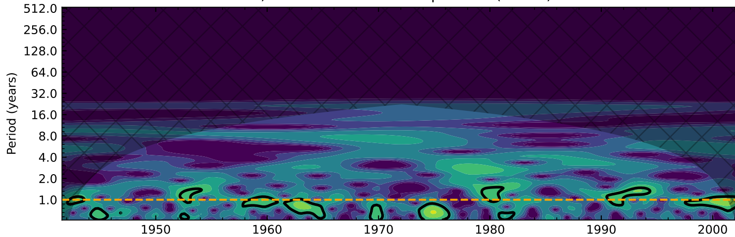
b) d13C Wavelet Power Spectrum (Morlet)
