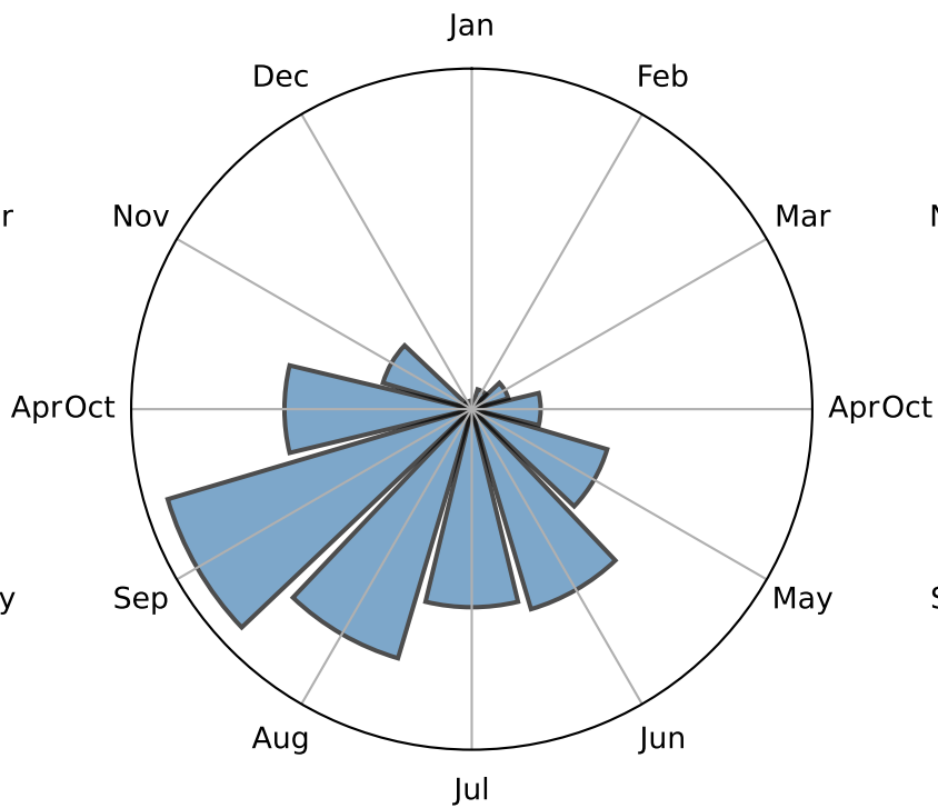
observed \delta^{18}\text{O}
