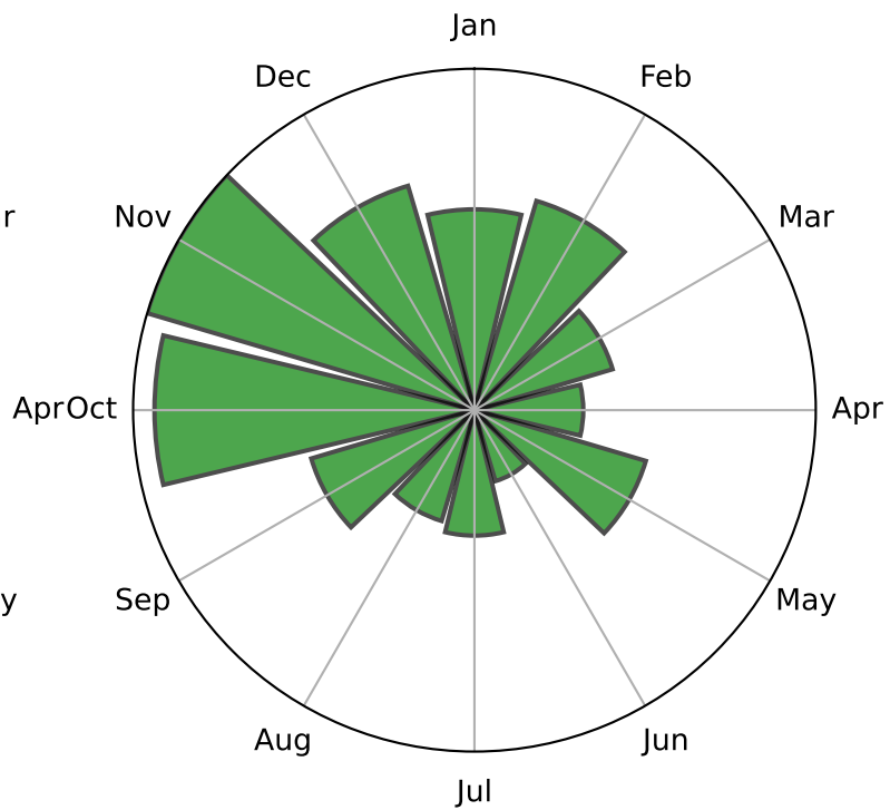
observed \delta^{13}\text{C}
