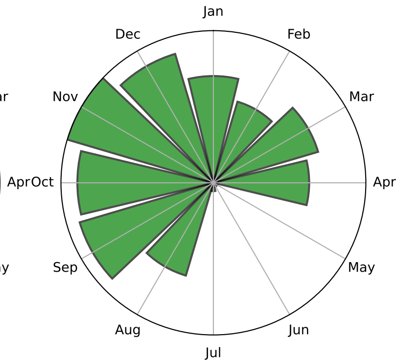
Observed \delta^{13}\text{C}
