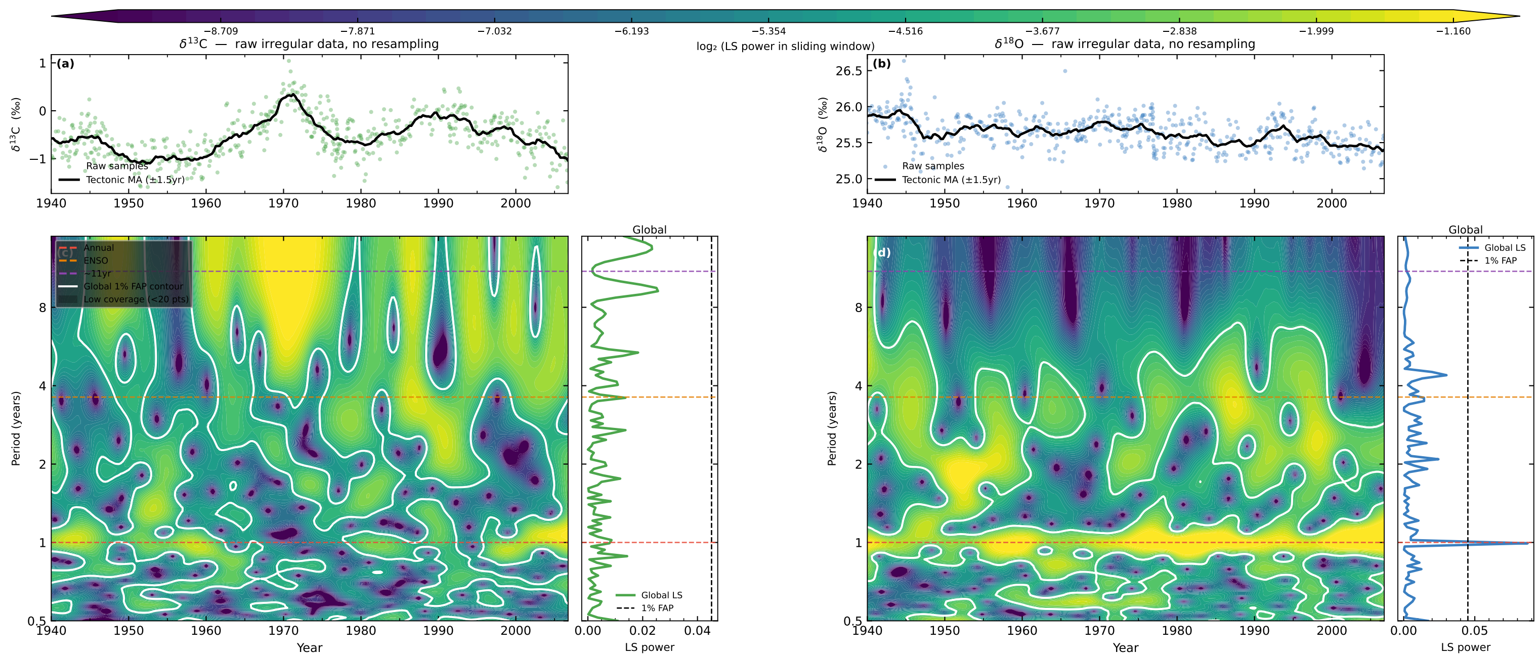
Sliding-window Lomb-Scargle (SWLS, \sigma=2.0\text{yr} Gaussian): weighted LS on raw irregular samples at each time grid point. No resampling. Tectonic removed via \pm 1.5\text{yr} time-based MA on raw data. White contour = global 1% FAP level (conservative local indicator).
