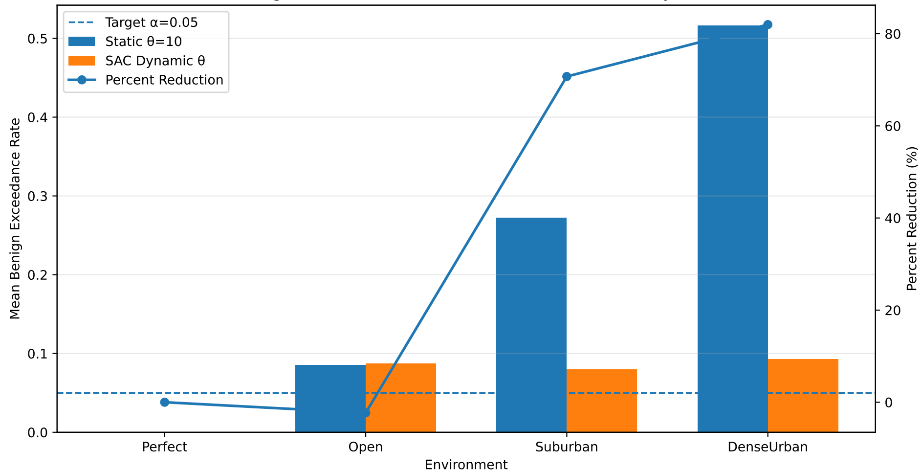
Figure 10: Final Static vs SAC Performance Summary
