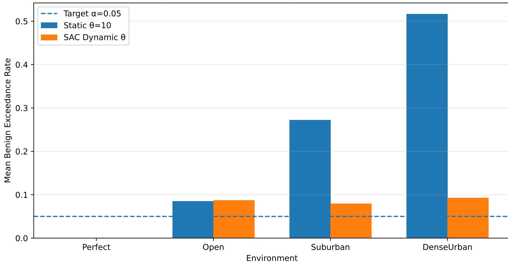
Figure 4: Static vs SAC Benign Exceedance Rate
