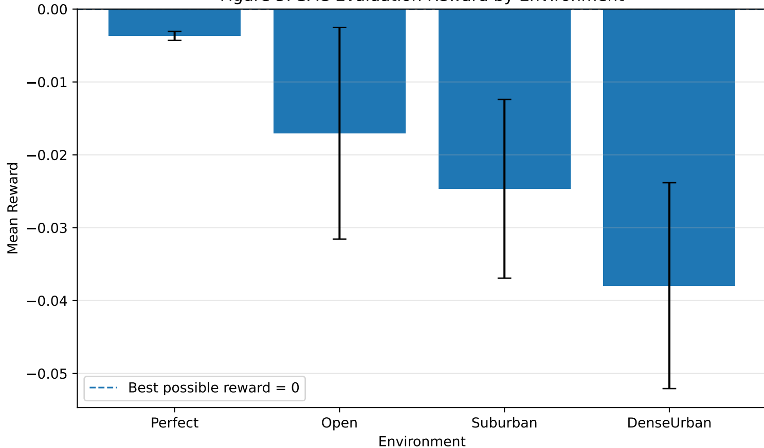
Figure 5: SAC Evaluation Reward by Environment
