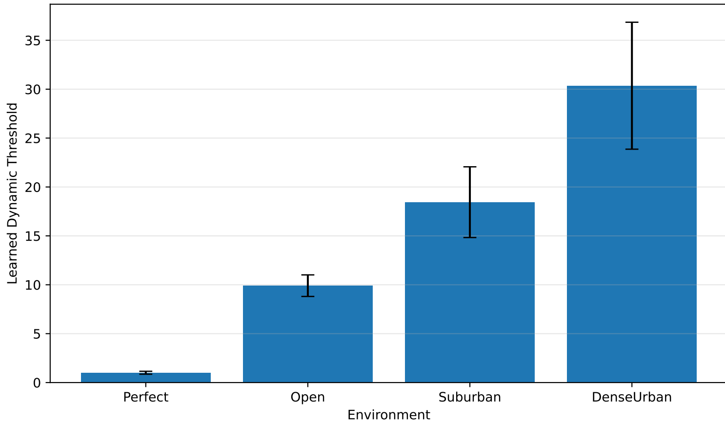
Figure 1: SAC Learned Threshold by Environment
