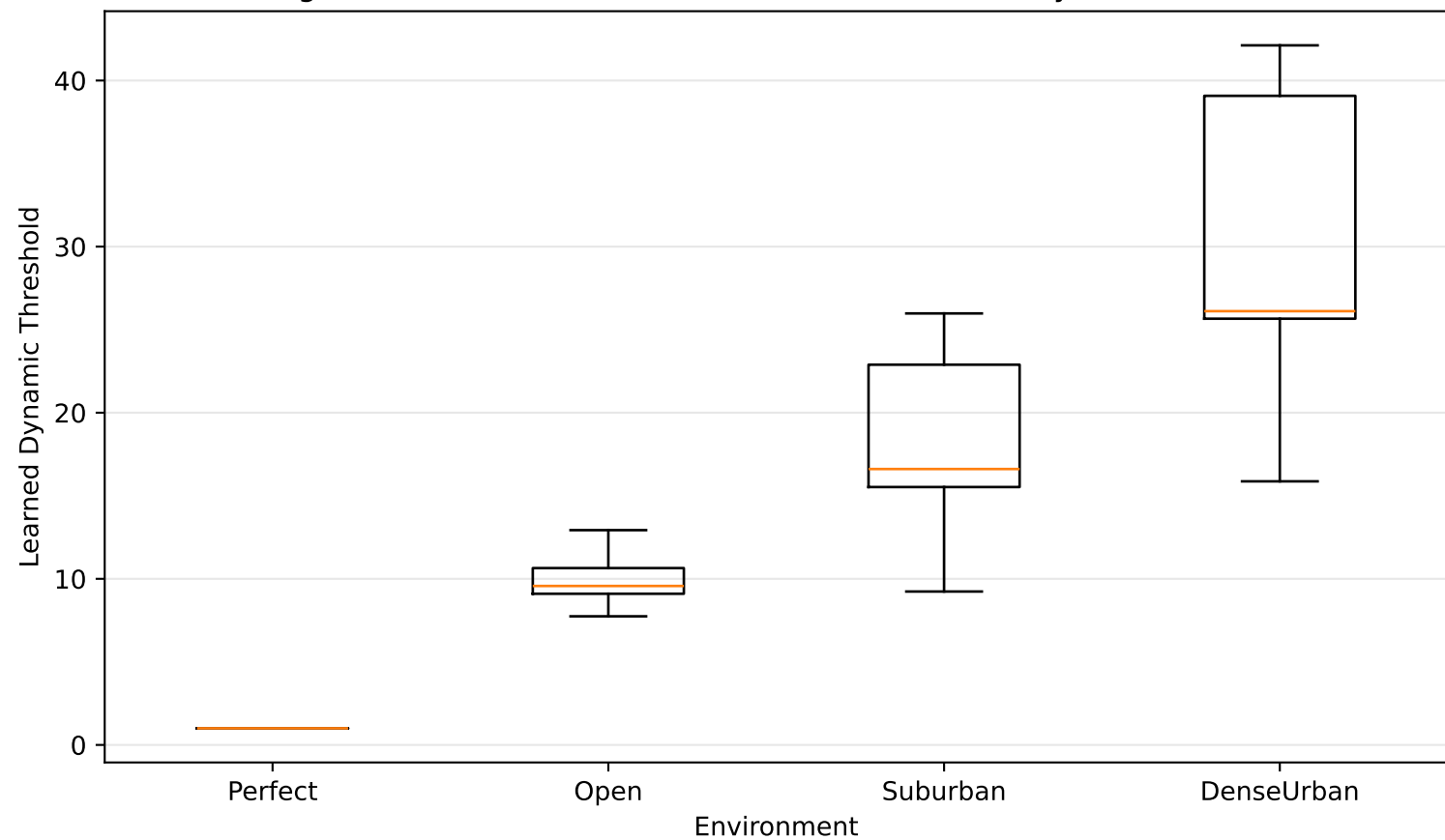
Figure 9: Distribution of SAC Learned Thresholds by Environment
