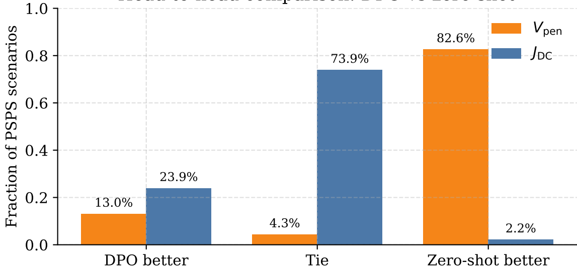
Head-to-head comparison: DPO vs zero-shot
