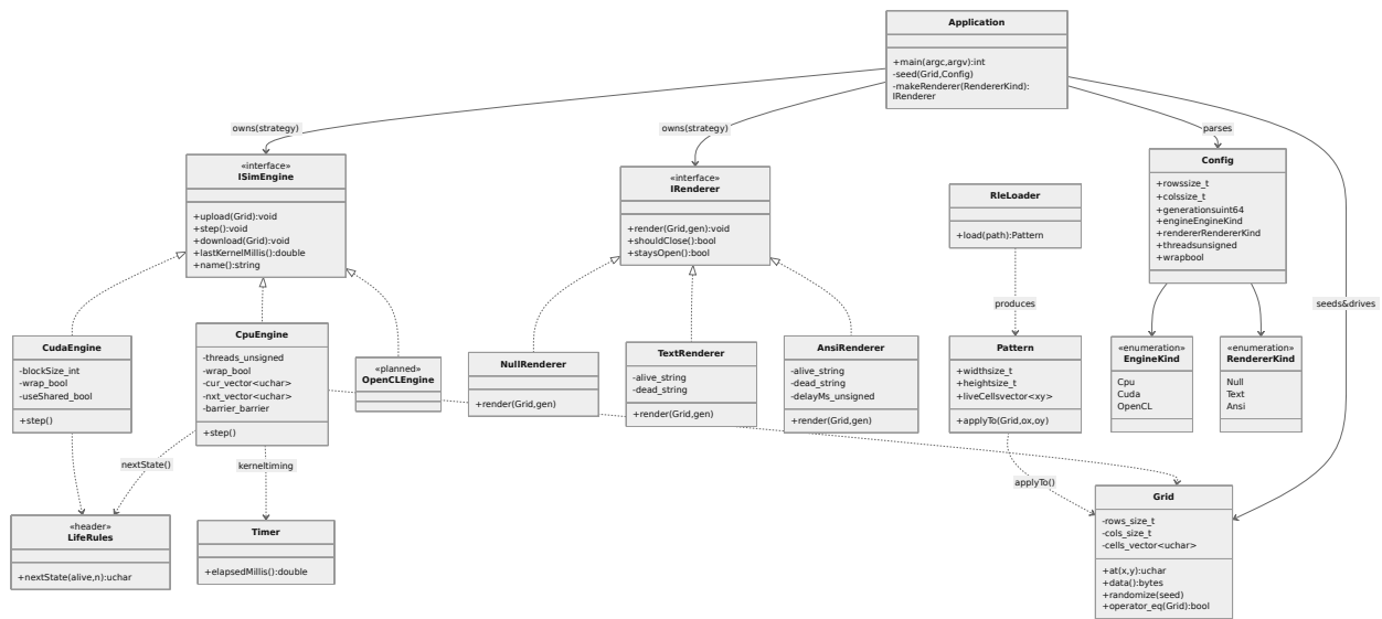
Figure 1: UML class diagram of the project (generated from report/diagrams/architecture.mmd with mermaid-cli ). The Application owns one ISimEngine and one IRenderer — the two strategy interfaces. CpuEngine and CudaEngine realize ISimEngine ; OpenCLEngine is marked planned . NullRenderer , TextRenderer and AnsiRenderer realize IRenderer . Dashed arrows are dependencies (e.g. CpuEngine and CudaEngine both use LifeRules::nextState ; RleLoader produces a Pattern that stamps a Grid ).
