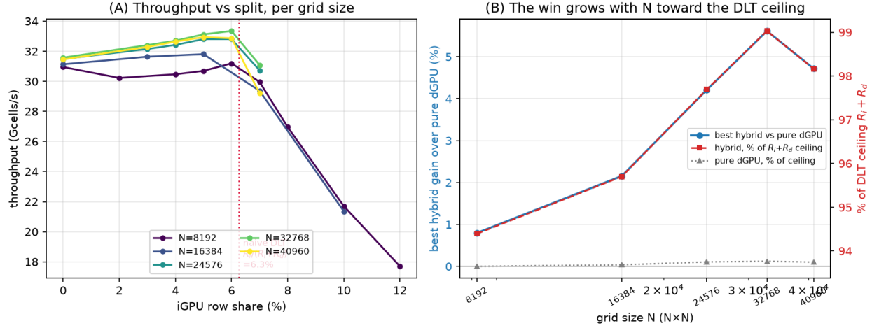
Figure 2: iGPU+dGPU fraction sweep. (A) Steady-state throughput vs the iGPU row share, one curve per grid size (best of five). Each curve rises to a peak near 5–6 % then falls off a cliff as the iGPU is overloaded past the dGPU’s step time; the empirical peak sits just below the naive-DLT share R_i/(R_i+R_d) \approx 6.3\% (dotted). (B) The best static split’s gain over pure dGPU (left axis) grows with N , and the hybrid’s share of the R_i + R_d ceiling (right axis) climbs from 94 % to 99 % while pure dGPU stays flat at \sim 94\% — the fixed one-row seam amortized against N^2 compute.
