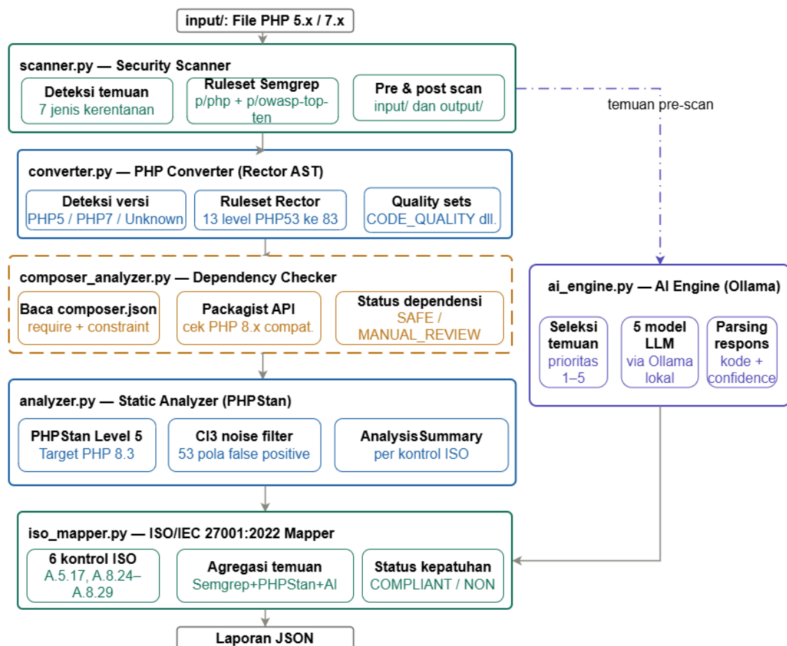
Gambar 3.3. Alur data pipeline : tahap masukan: Scanner, Converter, dan Composer Analyzer
