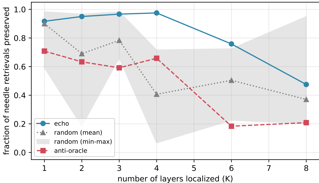
Retrieval-needle survival under localization (Qwen/Qwen2.5-0.5B-Instr) (120 retrievable needles)
