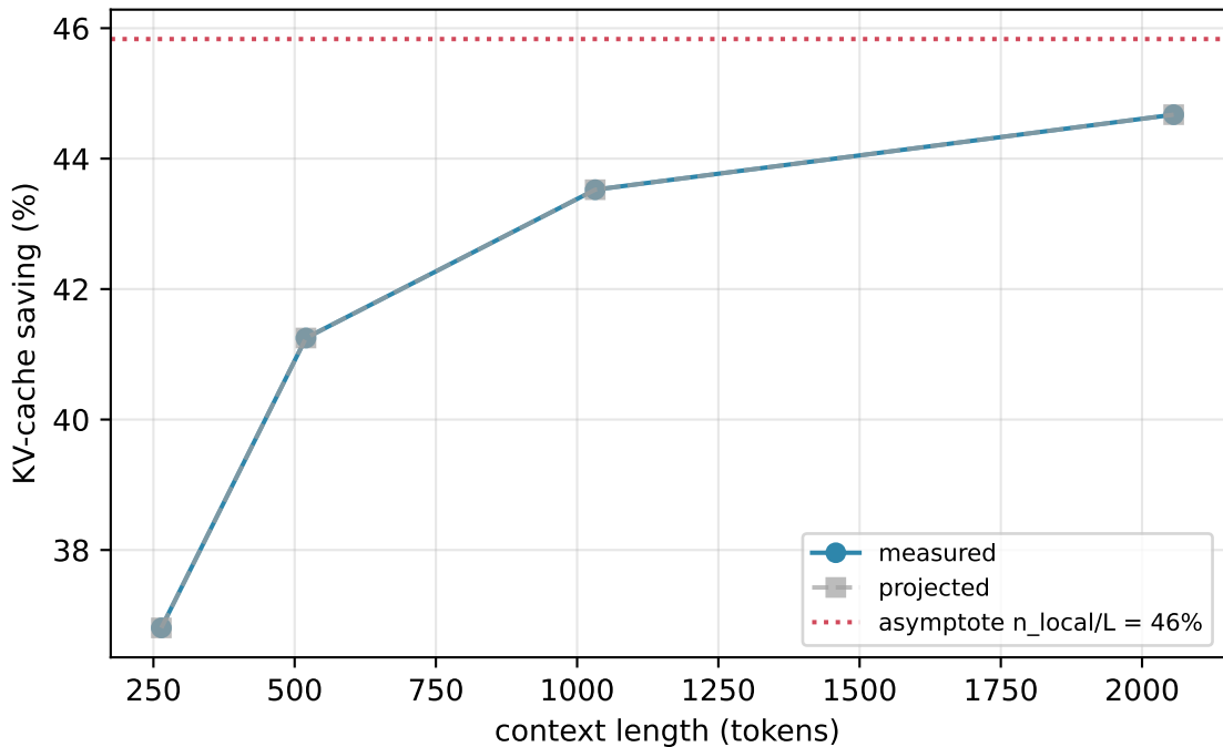
KV saving vs context (Qwen/Qwen2.5-0.5B-Instruct)
