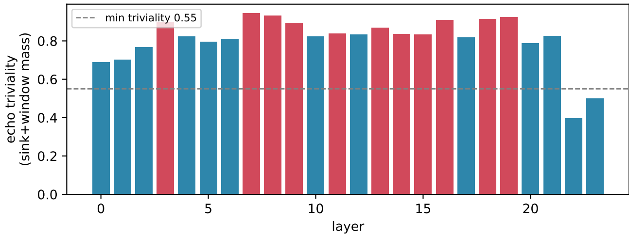
Per-layer echo triviality (11/24 localized, red)
