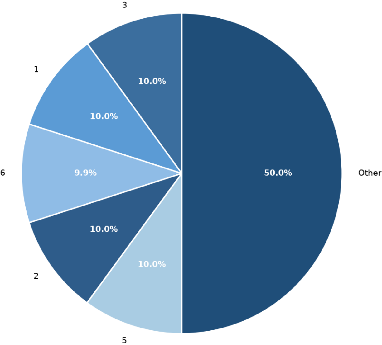
Average GPA by Department ID
