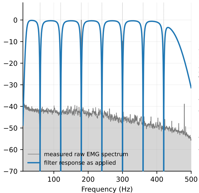
(b) Corrected chain: notch bank + bandpass
