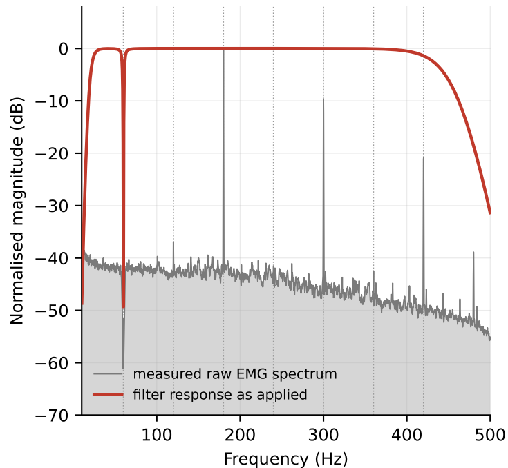
(a) Superseded chain: notch 60 Hz + bandpass
