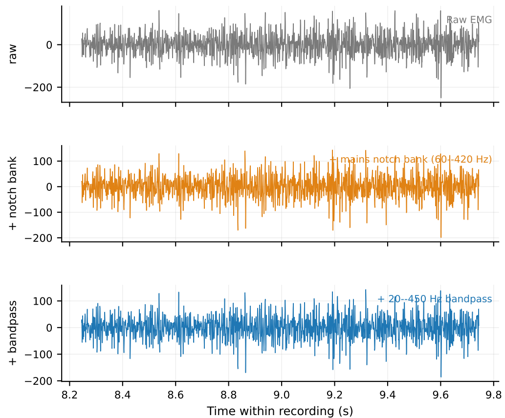
(a) left masseter, instructed clenching trial
