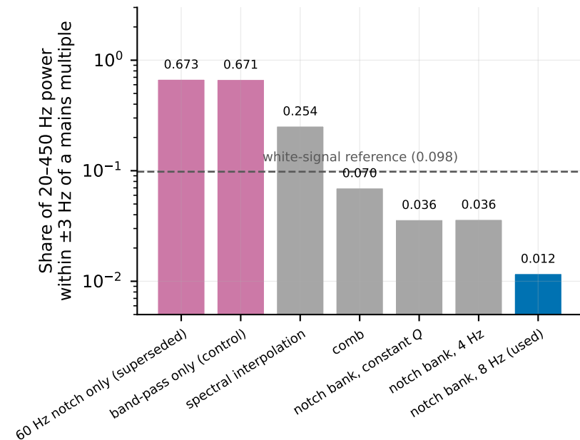
(c) The mechanism: interference was the signal
