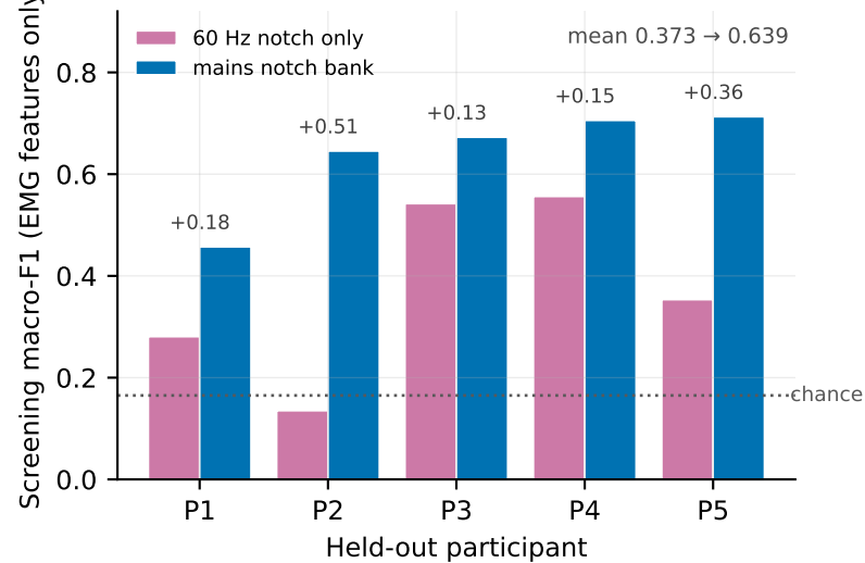
(b) The consequence for classification
