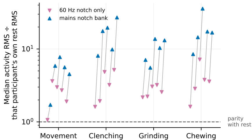
(c) The mechanism: interference was the signal
