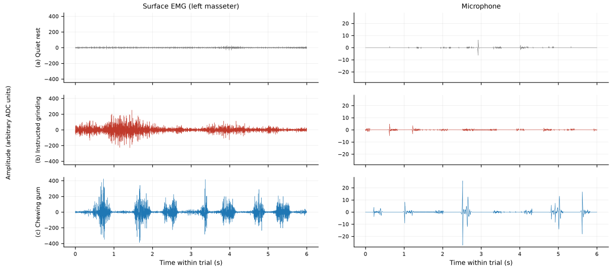
Fig. 12 Six-second excerpts of one participant’s quiet rest, instructed grinding, and gum chewing, after the corrected production filter chain, on a common scale within each column. (a) Rest is quiet in both channels. (b) Instructed grinding produces sustained EMG activation without a clear burst–relaxation rhythm, and comparatively little microphone energy. (c) Chewing produces rhythmic EMG bursts separated by relaxation intervals, alongside large microphone excursions; over the whole dataset the median filtered microphone RMS during chewing is 3.3 times that during instructed grinding (4.2 times in raw counts before filtering). The microphone row is not time-aligned with the EMG row above it, and the excursions are envelope-band rather than acoustic (Section 4.2). These excerpts are illustrative; they are not a measurement of the modality contribution.
