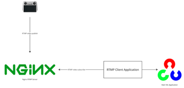
Figure 1: Process architecture for video ingest and deferred georeferencing.
