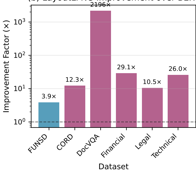
(b) LayoutLMv3 Improvement over BERT
