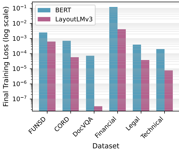
(a) Final Loss Comparison
