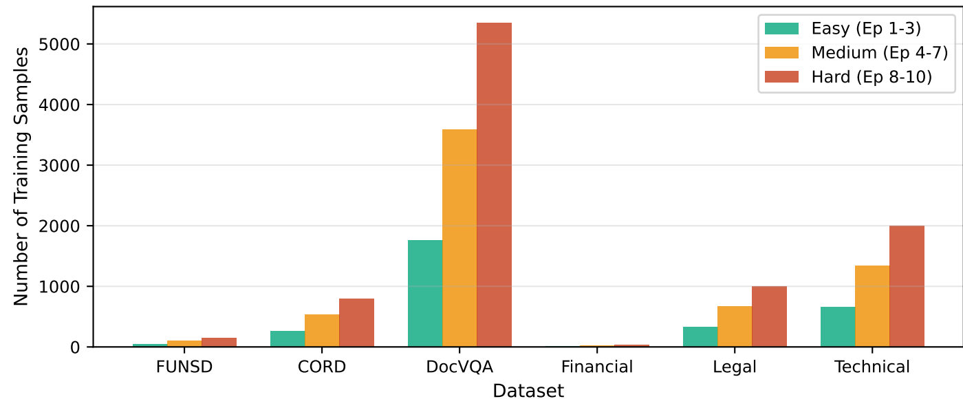
HCML Curriculum Learning: Sample Scaling Across Difficulty Phases
