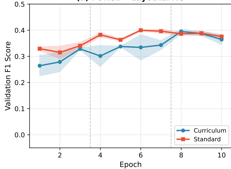
(a) FUNSD - LayoutLMv3
