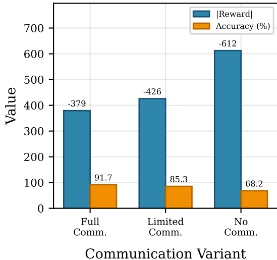
(a) Communication Ablation
