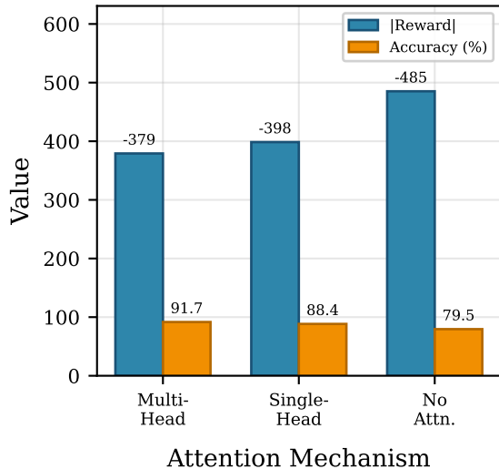
(b) Attention Ablation
