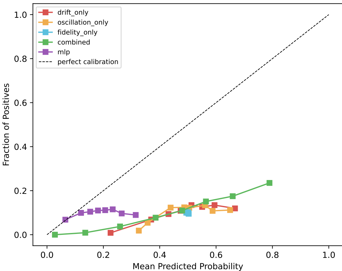
E5: Calibration Plot — k=5
