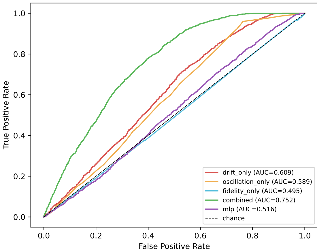
E5: ROC Curves — lead time k=5
