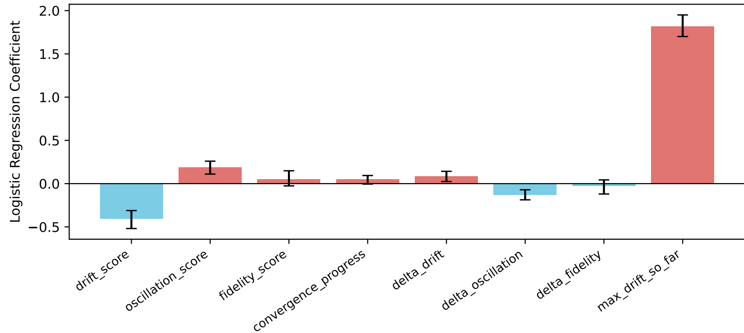
E5: Feature Importance (combined model, k=5, with 95% bootstrap CI)
