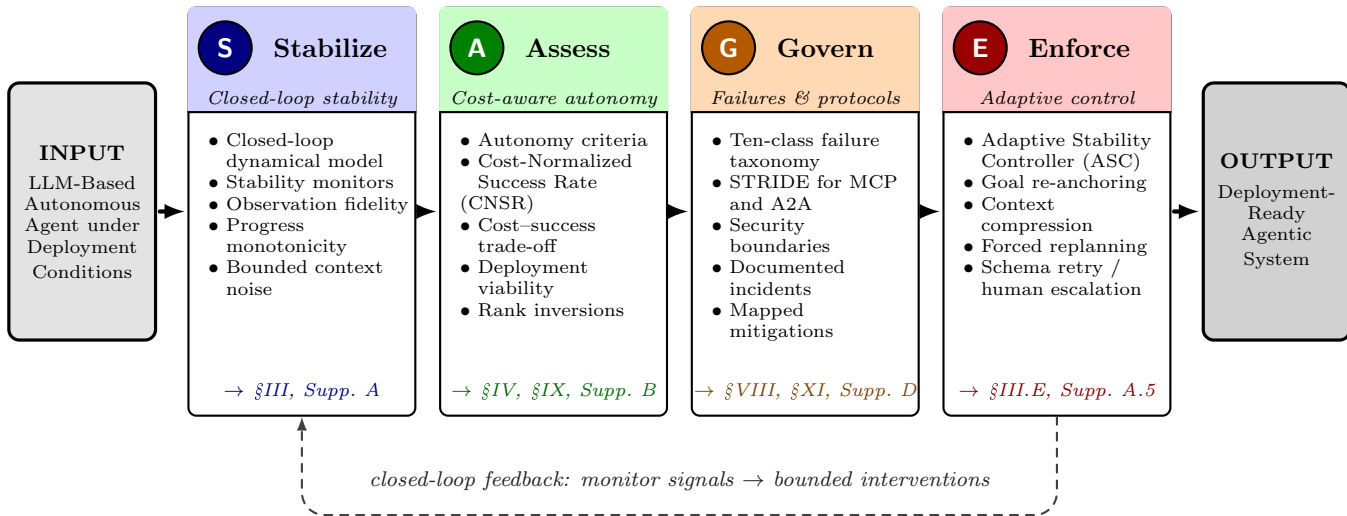
Figure 1: The SAGE framework for deployment-ready LLM-based autonomous agents.
