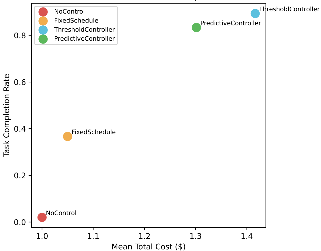
E4: Pareto — Cost vs. Completion
