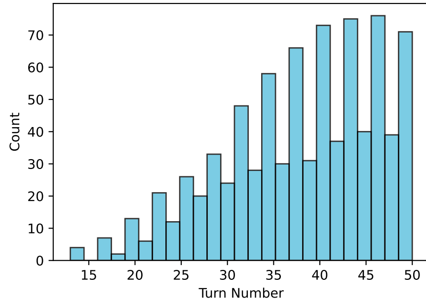
PredictiveController
