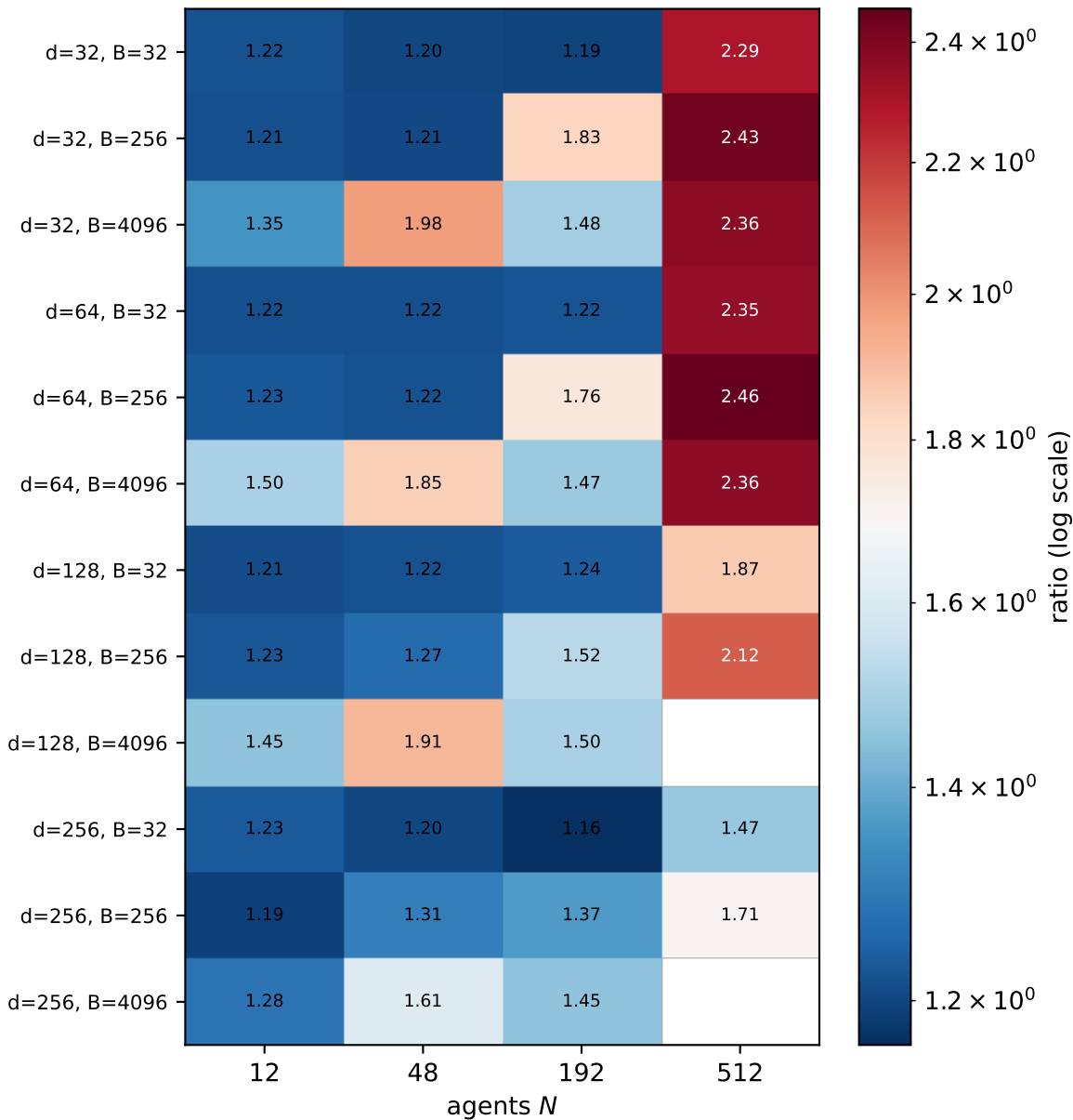
best- k gathered top- k latency \div dense (<1 = sparsity wins; blank = exceeded memory budget)
