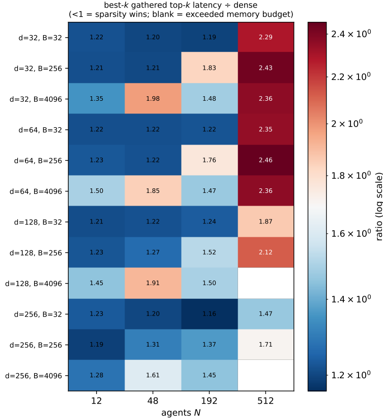
Figure 1: The crossover surface of Table 4. Every cell is > 1 : there is no operating point in the surveyed region at which a genuinely sparse top- k implementation is faster than dense attention. Blank cells exceeded the memory budget.
