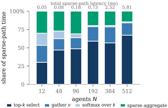
Selection dominates the sparse path
