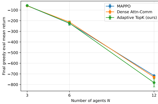
Figure 3: Final greedy-eval return vs N , error bars are across-seed std.
